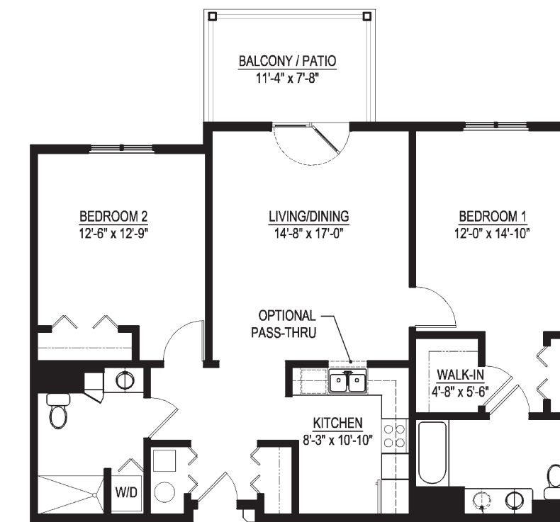
"D" - Two Bedroom — Apartment
