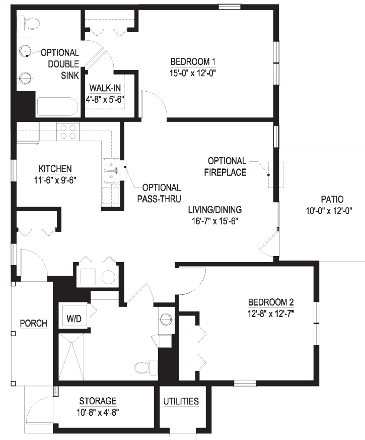
"H" - Two Bedroom — Cottage 1145 sq. ft. Approx.
